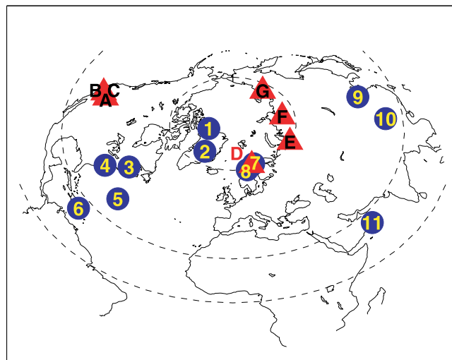
Figure 1 Locations of proxy data sites. Shown are the locations of eleven low-resolution proxy records (blue circles, numerals 1–11, see Table 1 for site details) and seven tree-ring series (red triangles, letters A–G). Dashed latitude lines indicate the Equator, the Tropic of Cancer and the Arctic Circle. See Supplementary Information for further details and references.
